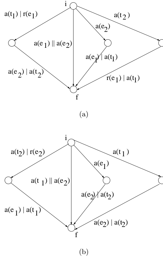
Fig. 3. Dependency automata: (a) Automaton for the dependency e_1 \rightarrow e_2 , (b) Automaton for the dependency e_1 < e_2
