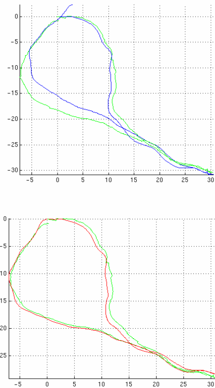
Figure 7 Top: Frame system of an extended outdoor run. Global pose from GPS and inertial sensors (green), frame system in blue. Note the overshoot at the end of the loop. Bottom: Frame system with loop closure, in red.
