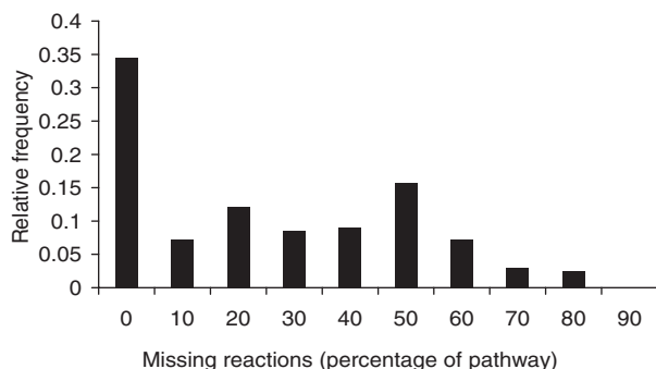
Figure 2. Distribution of incomplete pathways in VchoCyc based on the percentage of the reactions in a pathway that do not have assigned enzymes. For example, ~16% of the pathways in VchoCyc lack enzymes for 50% of their reactions.
