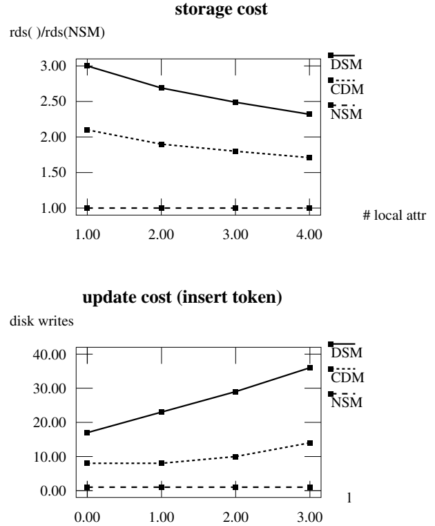
Fig. 5. a Storage and b update cost
