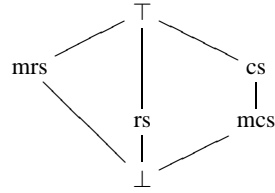
Figure 1. Simple hierarchy of closures. At the top of the lattice is the full closure, at the bottom the empty closure. Illustrated in the middle are a covering set (cs), a minimal covering set (mcs), a robust set (rs), and the most robust solution (mrs).
