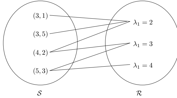
Figure 3. Solutions and realisations for Example 1.
