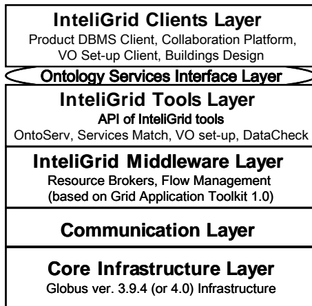
Figure 1. High level architecture of the IntelliGrid Ontology Services.
