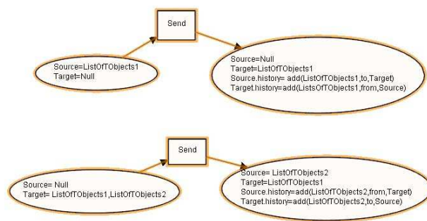
Figure 2: Execution Semantics from the perspective of the Sender
