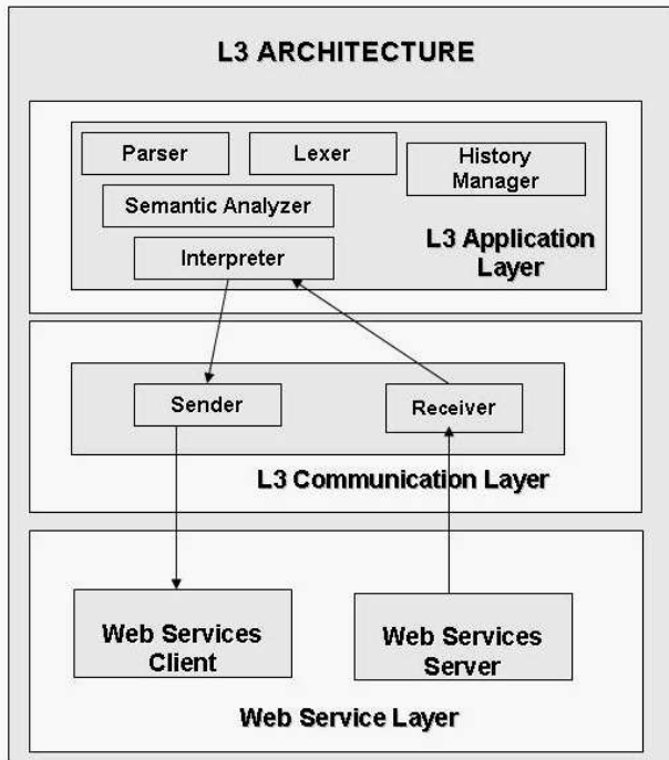
Figure 3: L3 Architecture
